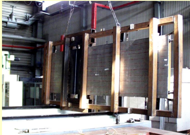
Beams of aircraft's wing. Alloy 7085
