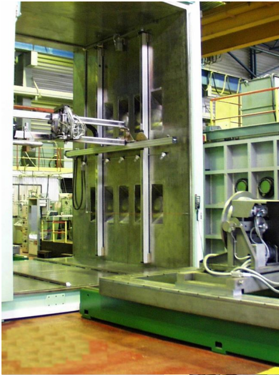
Example Of Our Projects: EBW Macine KL-118 For GKN Aerospace Chem-tronics Inc., USA
